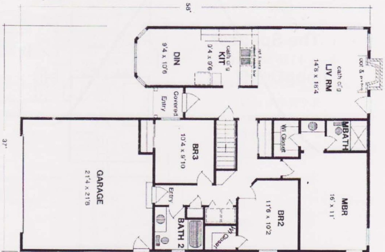
The Trowbridge Plan # 10-1348-1-A93-245 1348 Sq. Feet 3 Bed Room
